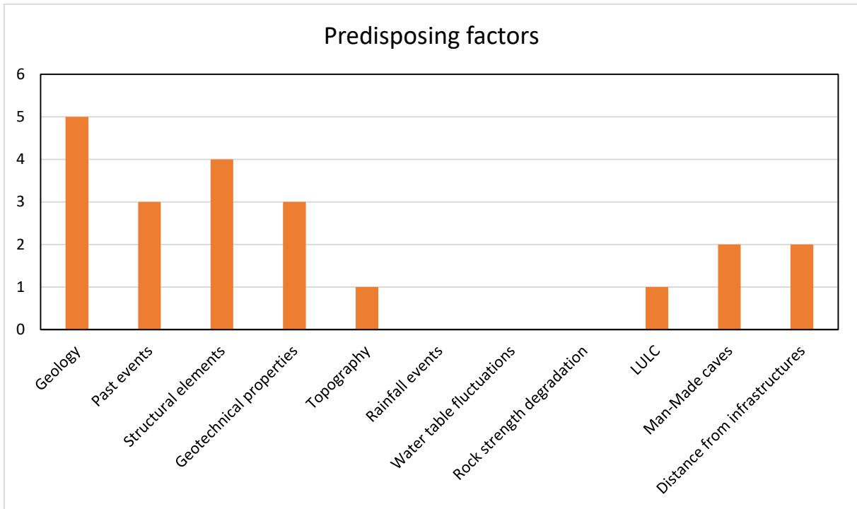
Figure 12: Graphs showing the predisposing factors characterizing the (rapid) sinkhole studies of the analyzed dataset.
