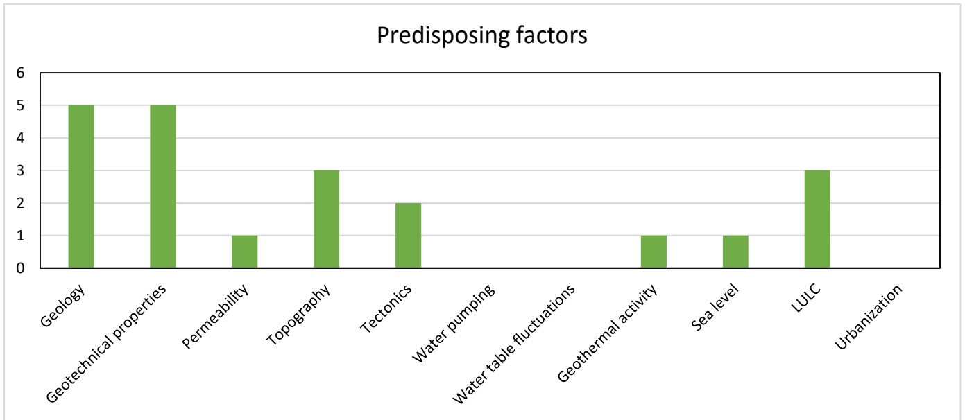
Figure 10: Graphs showing the predisposing factors characterizing the subsidence studies of the analyzed dataset.
