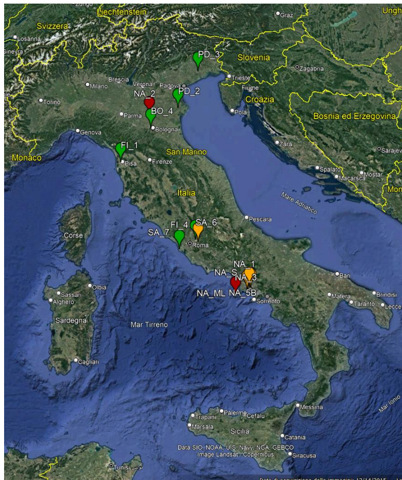
Figure 4: Location of the case studies composing the ground instabilities dataset (yellow: sinkholes; green: subsidence; red: liquefaction).
