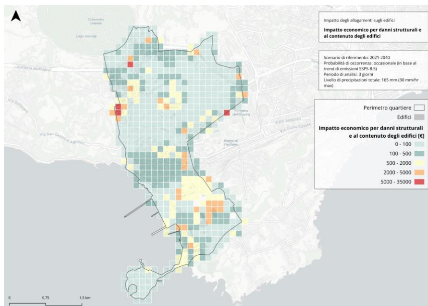
Figure 26. Economic impact due to structural and content damage to buildings resulting from a rainfall event of 165 mm over 3 days, with a peak intensity of 30 mm/hr, corresponding to an “occasional” scenario in the 2021–2040 period and a “frequent” one in the 2041–2070 period, based on the SSP5-8.5 emissions pathway
