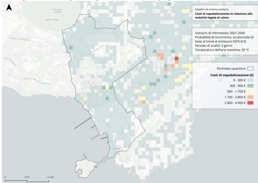
Figure 33. Estimated hospitalization costs associated with heat-stress-related conditions, based on a 3-day heat wave event with a peak air temperature of 39°C, with a probability of occurrence of "occasional" in the period 2021-2040 and "frequent" in the period 2041-2070 based on the SSP5-8.5 emissions trend. The map represents the scenario referring to the implementation of the actions identified by the project.
