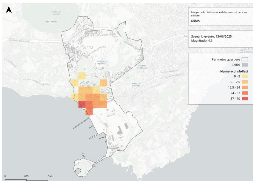
Figure 29. Estimated distribution of displaced residents resulting from a magnitude 4.6 earthquake that occurred on 13 June 2025. The map illustrates the situation as of June 2025
