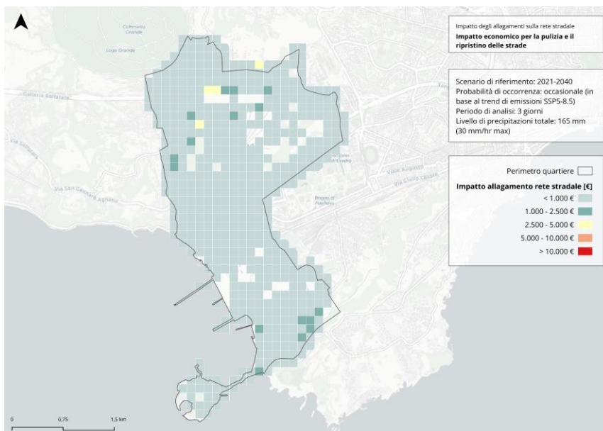
Figure 36. Economic impact of street cleaning and restoration following surface flooding events, associated with a rainfall event of 165 mm over 3 days, with a peak intensity of 30 mm/hr, corresponding to an “occasional” scenario for the period 2021–2040 and a “frequent” scenario for the period 2041–2070, based on the SSP5-8.5 emissions pathway. The map represents the scenario referring to the implementation of the actions identified by the project.
