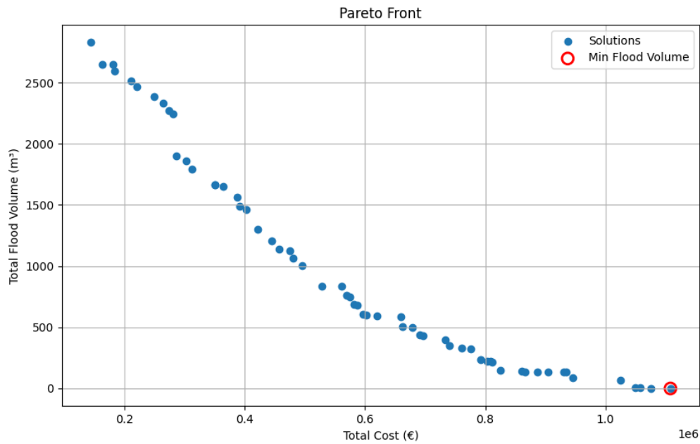
Figure 22 - Pareto Front of the entire set of solutions. The ante scenario gives more than 2500 m 3 of flooded volume, while the post scenario gives 0 m 3 flooded volume.
