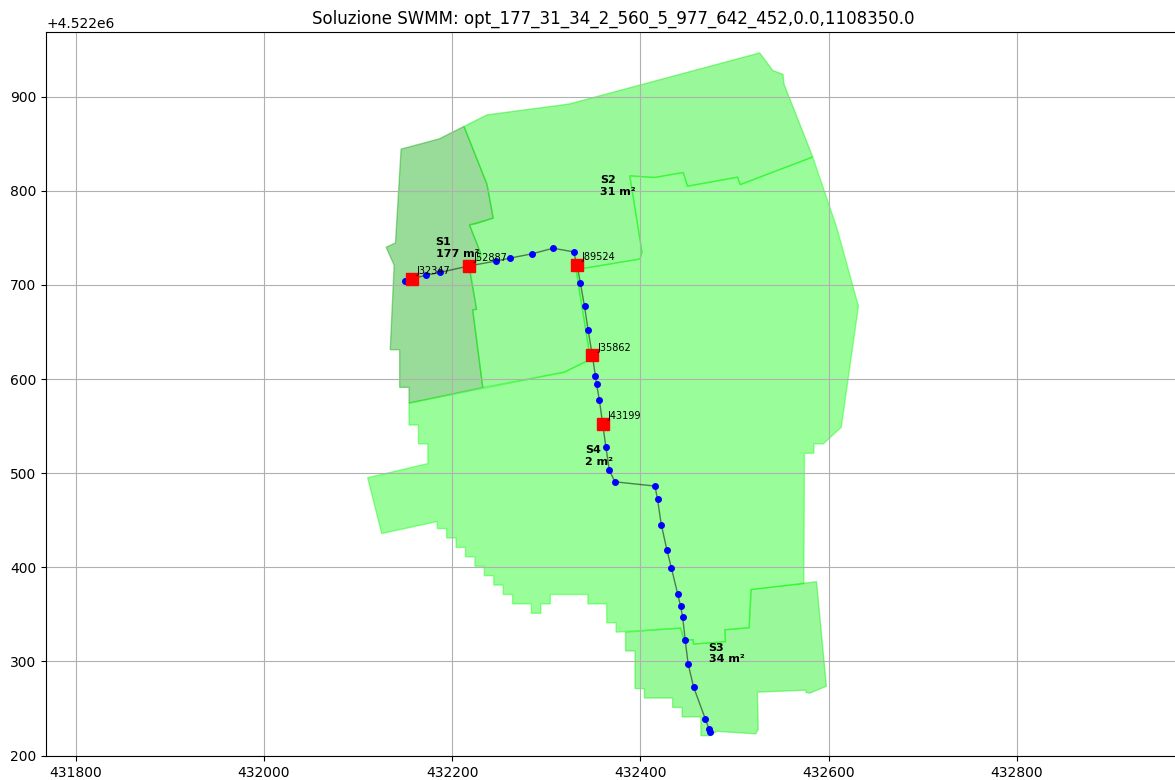
Figure 23 - Scenario post with the location of NBS+STORMWATER TANK solutions.
