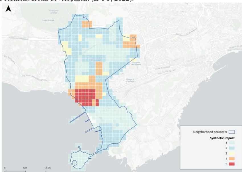
Figure 31. Synthetic impact map of the ex-ante scenario for the Bagnoli district. This map provides an integrated assessment of climatic and geophysical impacts at the urban scale, highlighting the most exposed and vulnerable elements under current conditions. It combines estimates of healthcare costs from
