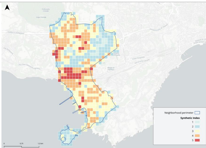
Figure 32. Synthetic Index of ex-ante multi-risk conditions in the Bagnoli district. The index integrates climate hazard indicators with geophysical impact estimates, providing a unified representation of areas where urban elements are most exposed and vulnerable. It reflects the potential intensity of heatwaves and pluvial flooding alongside expected losses from seismic and volcanic events, supporting the identification of priority areas for integrated multi-risk interventions and informing strategies for climate adaptation and disaster risk reduction.
