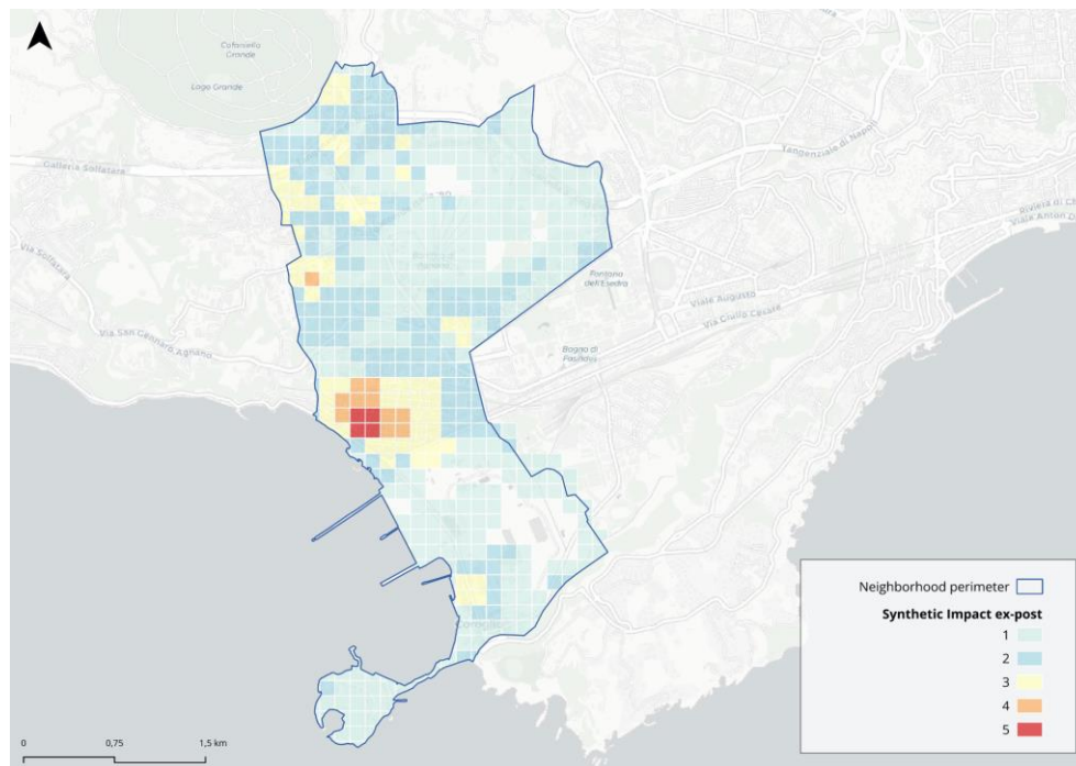
Figure 39. Synthetic impact map of the ex-post scenario for the Bagnoli district. The map provides an integrated assessment of residual multi-risk conditions following the implementation of combined urban interventions. It highlights the reduced expected impacts on buildings, open spaces, and population. It reflects the enhanced resilience achieved through the synergy of energy efficiency, climate adaptation, and structural safety measures. This overview supports the evaluation of intervention effectiveness and the prioritization of further multi-risk strategies.
