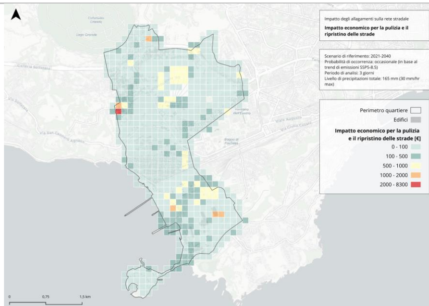
Figure 27. Economic impact of street cleaning and restoration following surface flooding events, associated with a rainfall event of 165 mm over 3 days, with a peak intensity of 30 mm/hr, corresponding to an “occasional” scenario for the period 2021–2040 and a “frequent” scenario for the period 2041–2070, based on the SSP5-8.5 emissions pathway.
