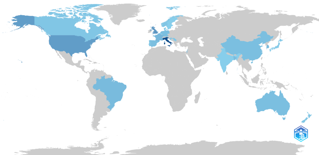
Figure 1. Country Scientific Production (Images are the result of the data analysis conducted on R-Studio to A. Rocco versus scientific evidence and cannot be substituted)
