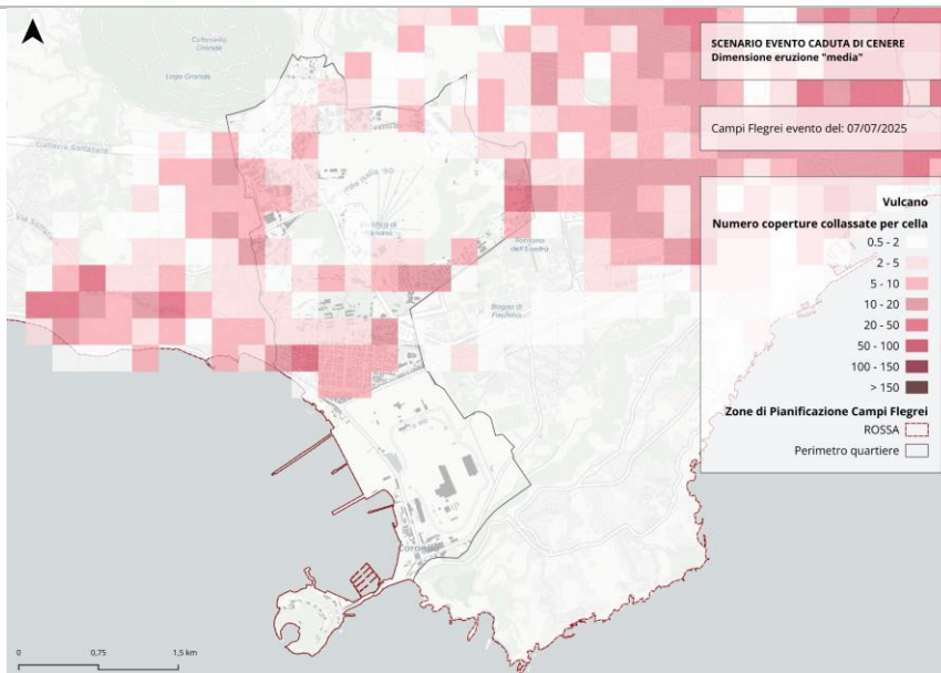
Figure 30. Estimated number of roof collapses caused by ash fallout from a medium-size eruptive event at the Campi Flegrei volcanic area on 07 July 2025. The map illustrates the resulting impacts on building structures across the affected area
