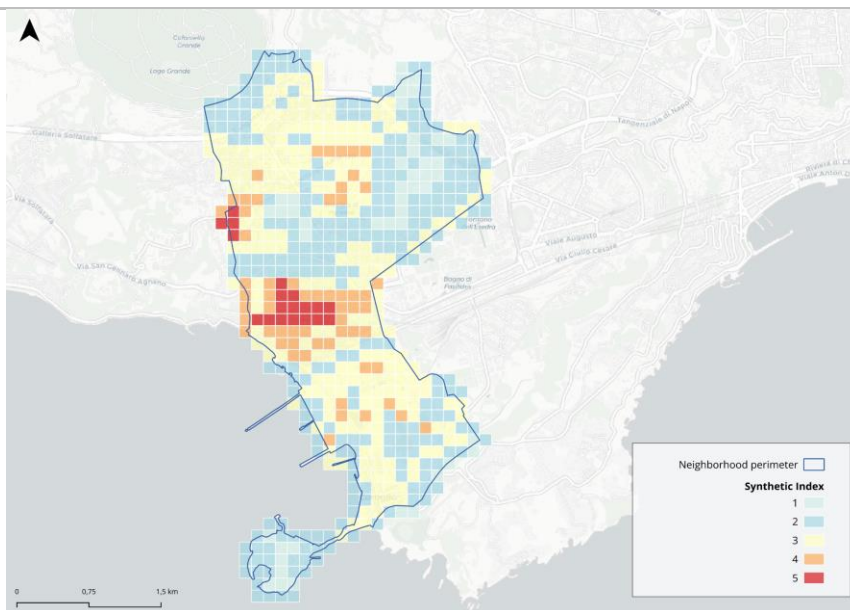
Figure 40. Ex-post Synthetic Index of multi-risk conditions in Bagnoli. The index combines updated climate hazard and geophysical impact indicators, reflecting the effects of implemented interventions on buildings and open spaces.
