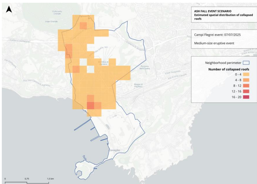
Figure 38. Estimated number of roof collapses caused by ash fallout from a medium-size eruptive event at the Campi Flegrei volcanic area on 07 July 2025 following the implementation of the proposed actions. The map illustrates the expected impacts on building structures after project implementation, showing a reduction in roof collapses compared to current conditions, based on the same data and methodology.
