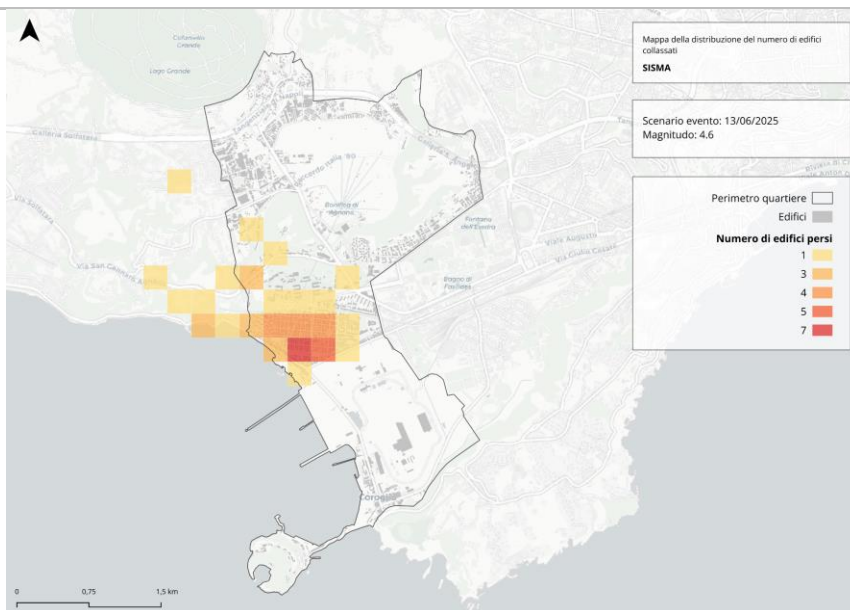
Figure 28. Estimated distribution of collapsed buildings resulting from a magnitude 4.6 earthquake that occurred on 13 June 2025. The map illustrates the situation as of June 2025
