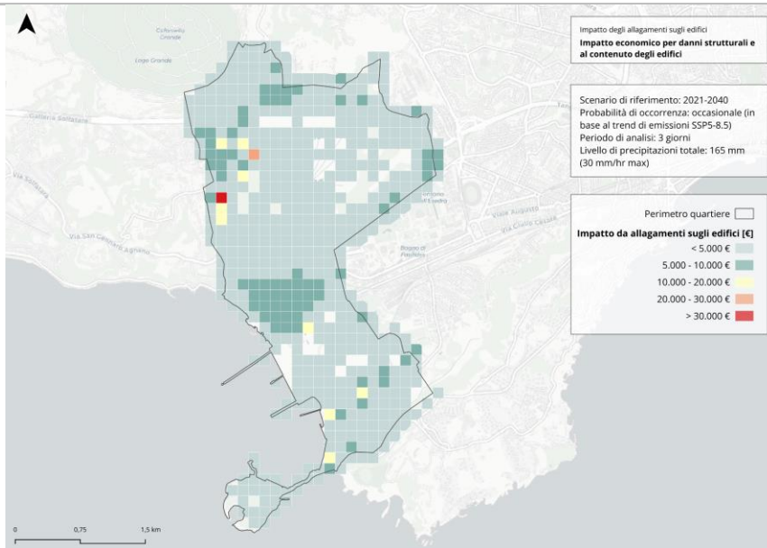
Figure 35. Economic impact due to structural and content damage to buildings resulting from a rainfall event of 165 mm over 3 days, with a peak intensity of 30 mm/hr, corresponding to an “occasional” scenario in the 2021–2040 period and a “frequent” one in the 2041–2070 period, based on the SSP5-8.5 emissions pathway. The map represents the scenario referring to the implementation of the actions identified by the project.
