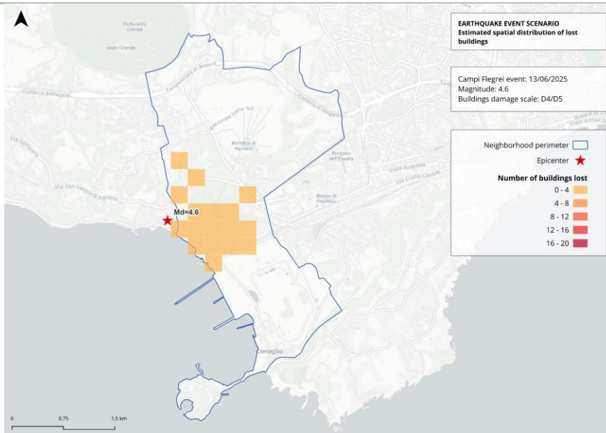
Figure 37. Estimated distribution of collapsed buildings resulting from a magnitude 4.6 earthquake of 13 June 2025 following the implementation of the proposed actions. The map illustrates the expected impacts after project implementation, showing a reduction in the number of collapsed buildings compared to the current conditions, based on the same data and methodology.
